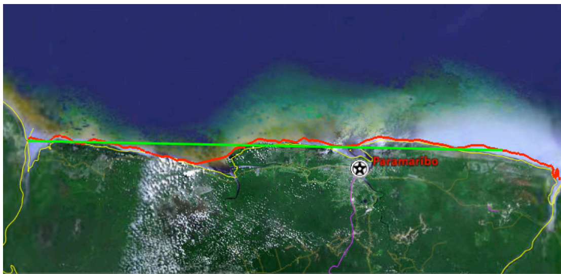
Figure 2. Area-balance line for Suriname. The red curve is define by the low-tide points for Suriname that are given in Table 2. The green line is the area-balance line.
